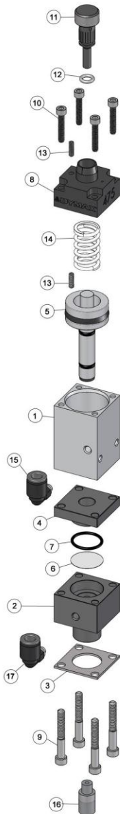
Figure 4. Model 475 Replacement Parts
