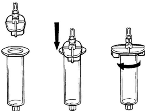
Figure 4. Barrel and Air Cap Assembly Lock Procedure
