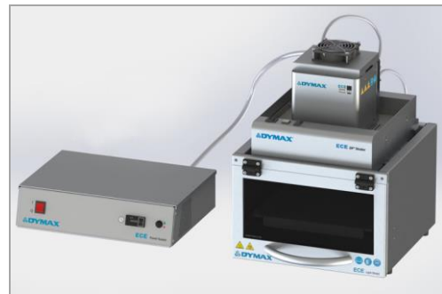
ECE 5000 flood system mounted on shutter with a light shield
