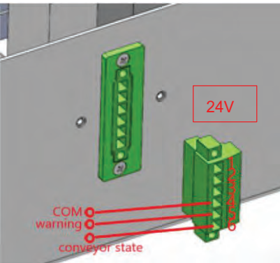
Figure 62. Status Outputs Connection to Customer's Monitor Device
