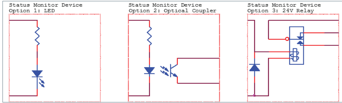
Figure 63. Examples of Customer Configurations for Monitoring Outputs
