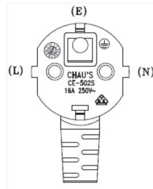
Figure 31. Power Cord with TYPE-F EU Plug
