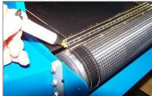
Figure 22. Applying Adhesive
