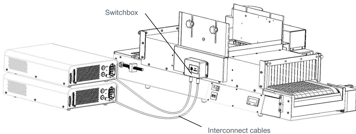
Figure 5. Connect Footswitch to Switchbox
