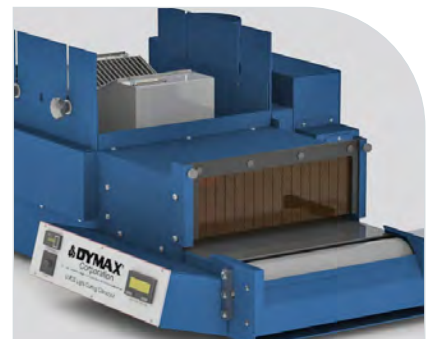
Two LED Floods Mounted in a UVCS Conveyor
