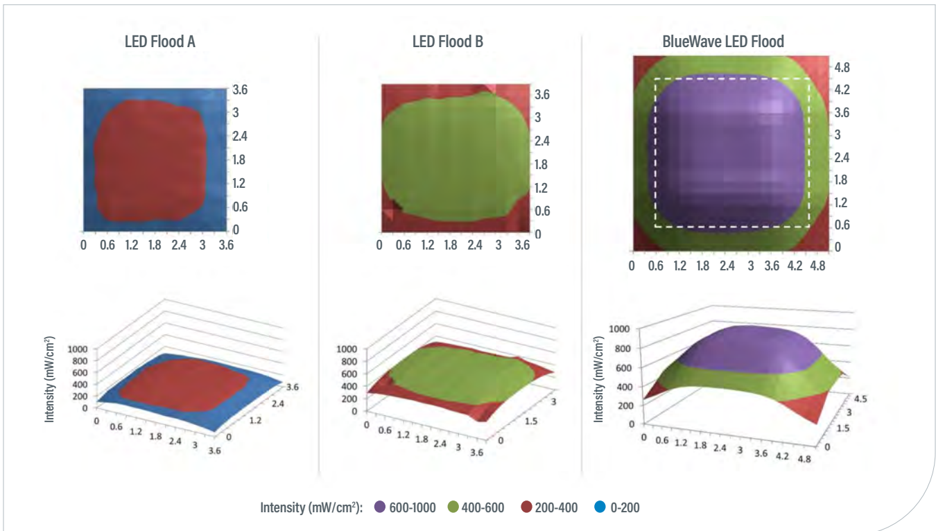
Figure 2. Curing Uniformity
