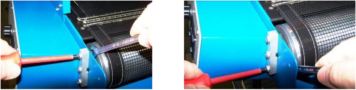
Figure 20. Loosening Drive-Roller Shaft-Support Fasteners
