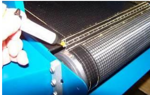
Figure 19. Applying Adhesive
