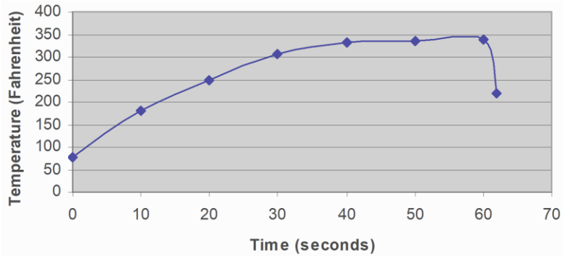
5000-EC Flood Lamp (135 mw/sqcm) on Black Polymer Surface
