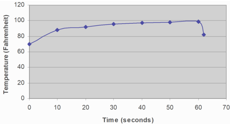
2000-EC Flood Lamp on Black Polymer Surface
