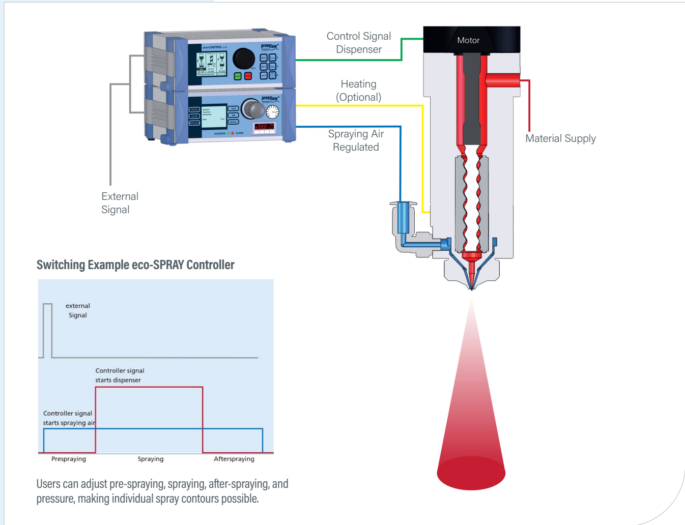
Figure 3. eco-SPRAY System
