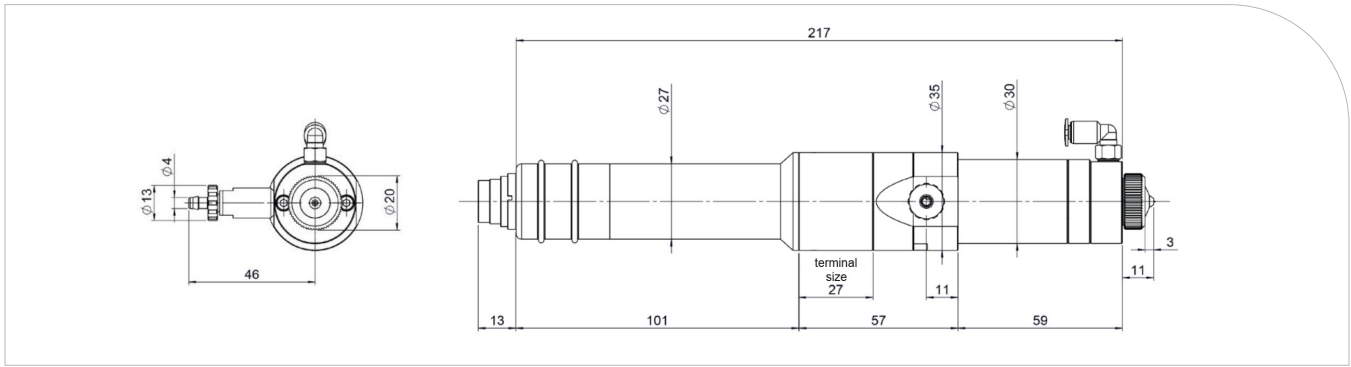
Figure 1. eco-SPRAY Dimensions
