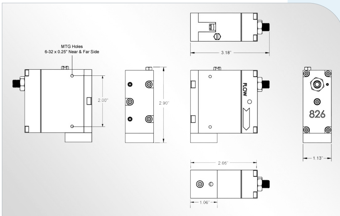
Figure 1. Model 826 Dimensions
