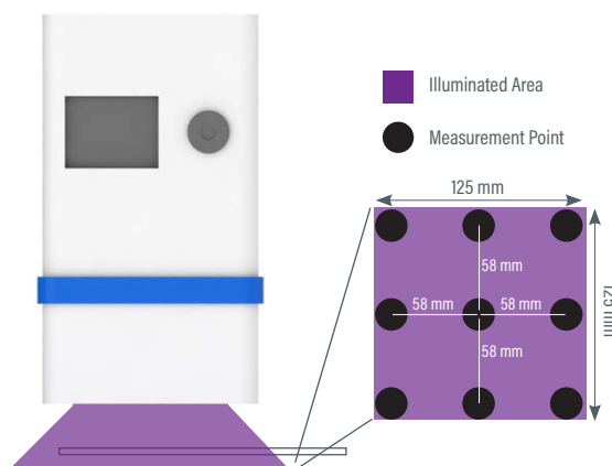
Figure 6. Example of Measurement Location of the Radiometer at a Fixed Working Distance to Determine the Uniformity
