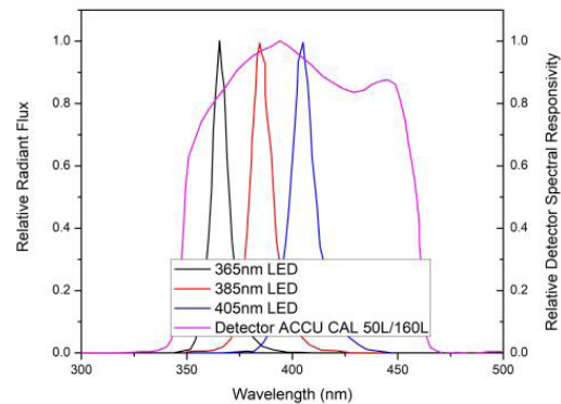
B. Detector spectrum of ACCU-CAL™ 50-LED / ACCU-CAL™ 160 LED and Spectrum of UV LEDs
