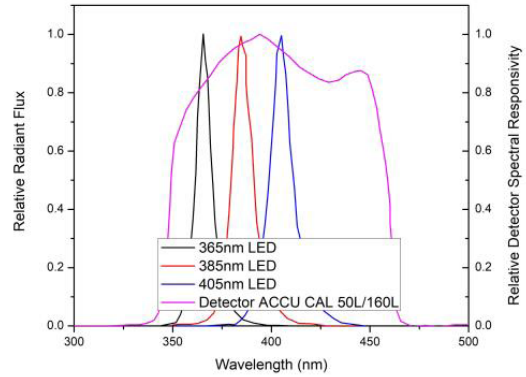
A. Detector spectrum of ACCU-CAL™ 50 / ACCU-CAL™ 160 and Spectrum of Metal-Halide and Mercury Lamps.
