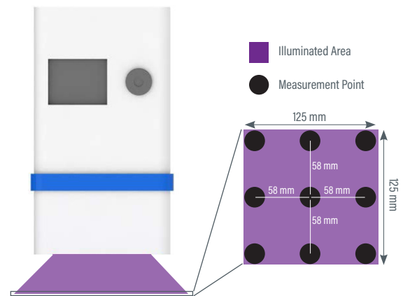
Figure 6. Example of Measurement Location of the Radiometer at a Fixed Working Distance to Determine the Uniformity
