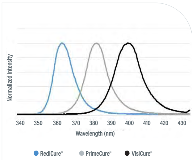
Figure 2. BlueWave AX-550 V2.0 Emitter Spectral Output Chart
