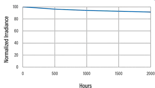
Figure 5. LED Degradion Testing - RediCure®
