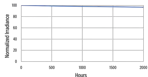
Figure 6. LED Degradion Testing - PrimeCure®
