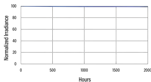
Figure 7. LED Degradion Testing - VisiCure®
