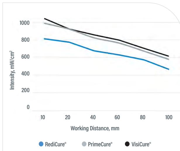
Figure 3. BlueWave® AX-550 V2.0 Emitter Relative Intensity vs. Distance
