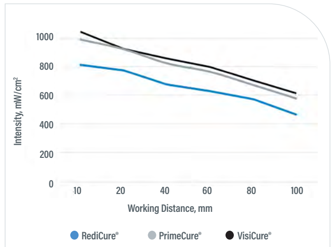
Figure 3. BlueWave® AX-550 V2.0 Emitter Relative Intensity vs. Distance
