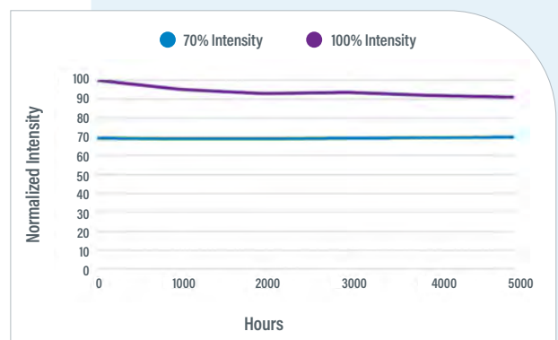
Figure 11. LED Degradion Testing - VisiCure
