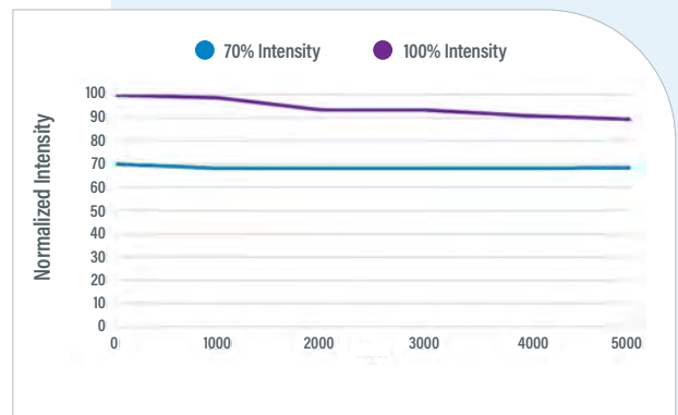
Figure 10. LED Degradion Testing - PrimeCure
