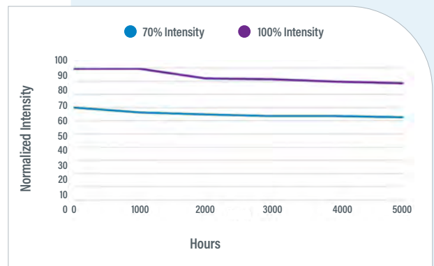
Figure 9. LED Degradion Testing - RediCure
