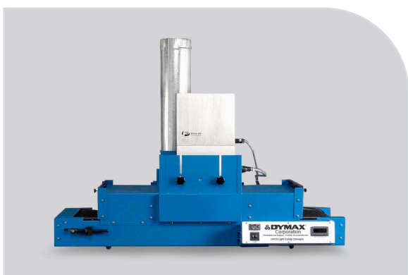
UVCS conveyor with one center-mounted Fusion
