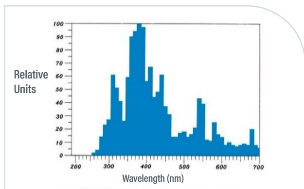
Spectral distribution with a metal-halide, iron-doped mercury bulb PN 41247
