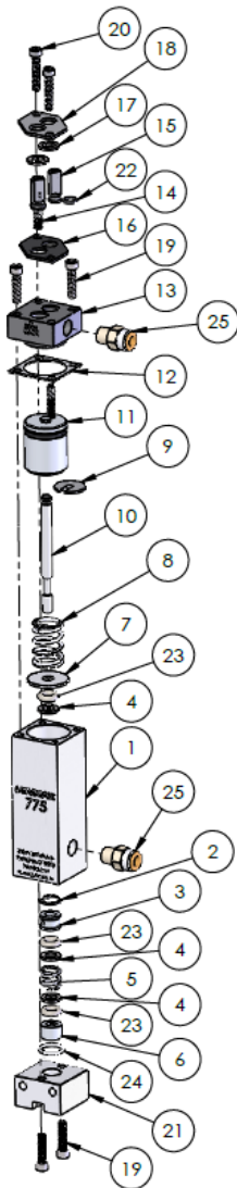
Figure 5. 775 Replacement Parts
