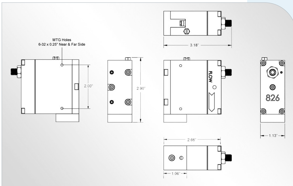
Figure 1. Model 826 Dimensions
