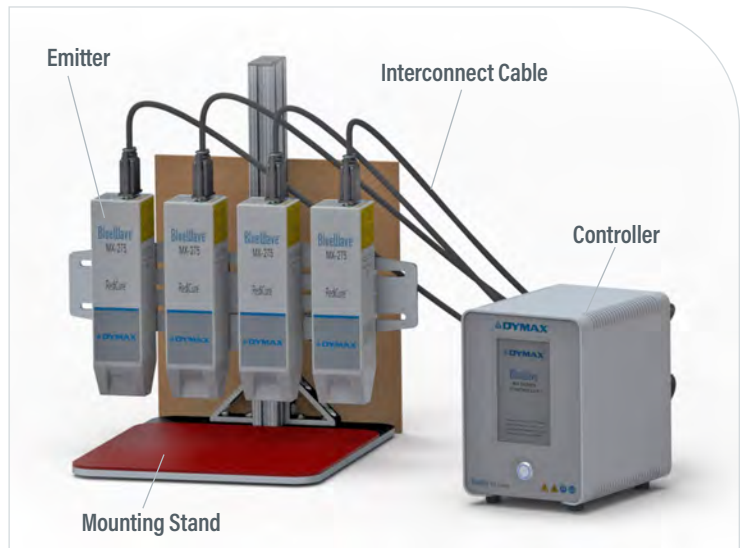
Figure 2 BlueWave MX-275 System Components
