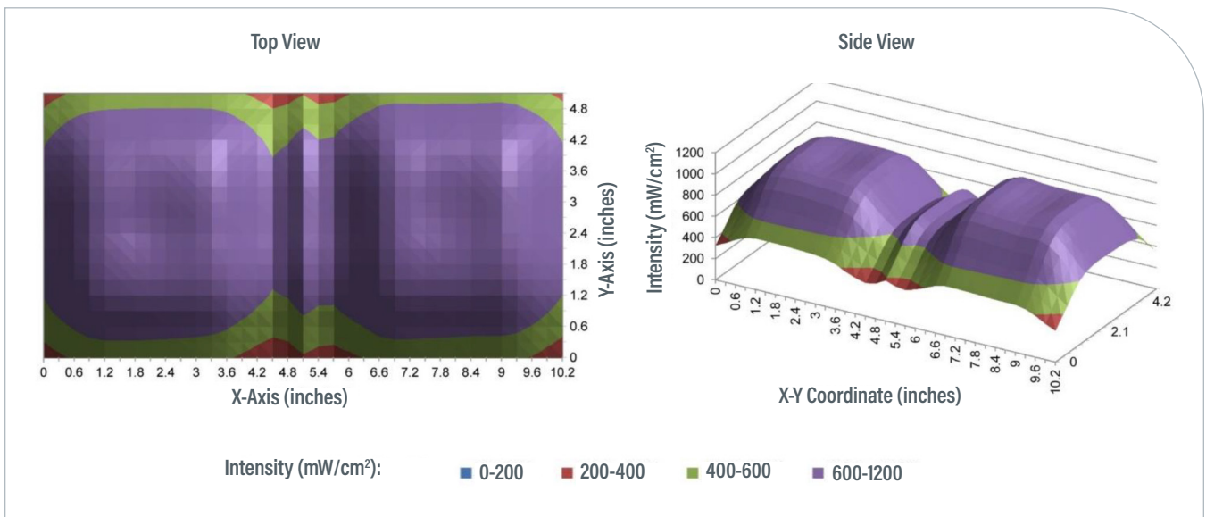
Figure 1. Intensity Distribution of Two BlueWave LED Flood VisiCure Arrays (405 nm) Mounted Side-by-Side
