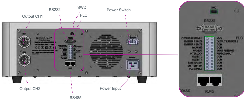
Figure 9. Controller Connections
